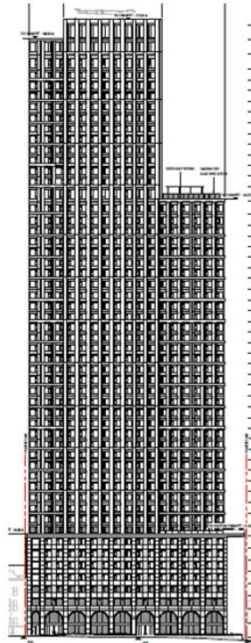
West elevation
