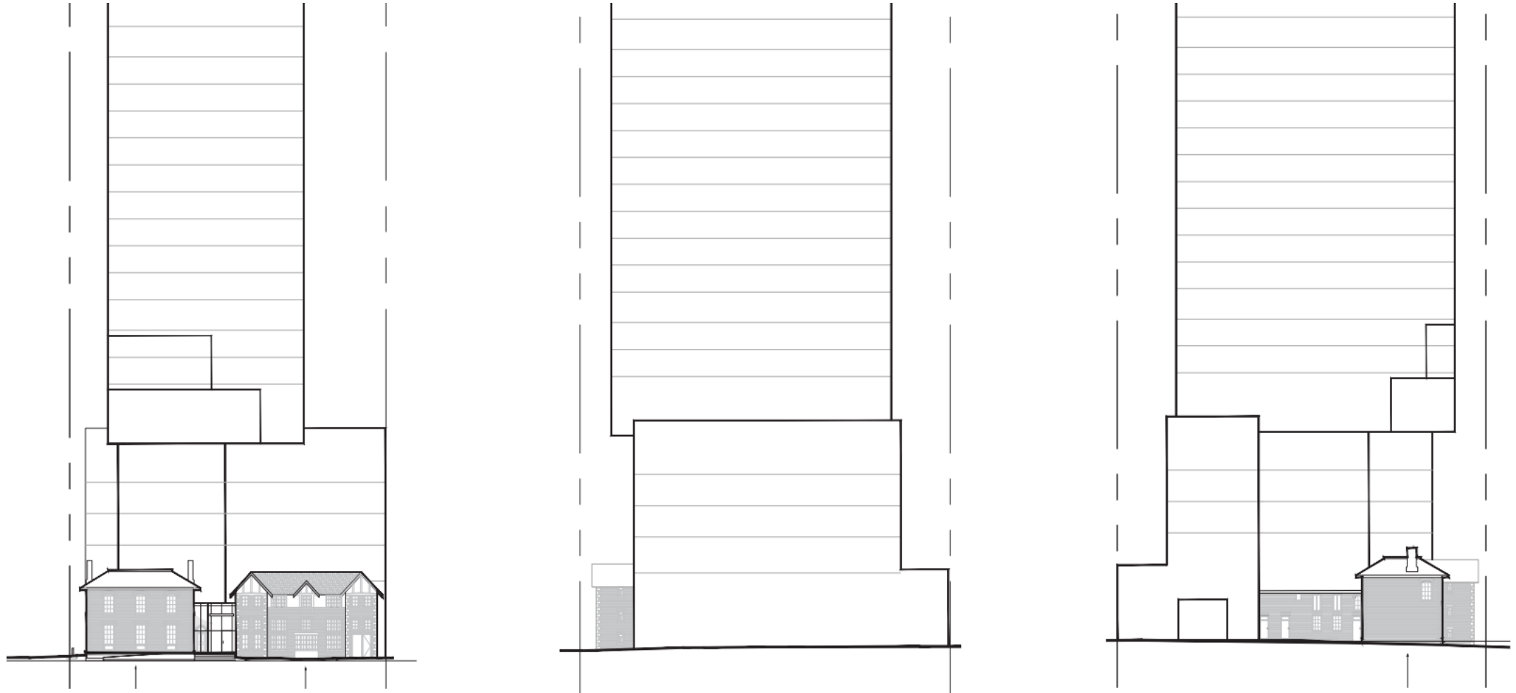
North, west, and south elevation plans of the proposed development (BDP Quadrangle, 2024)
