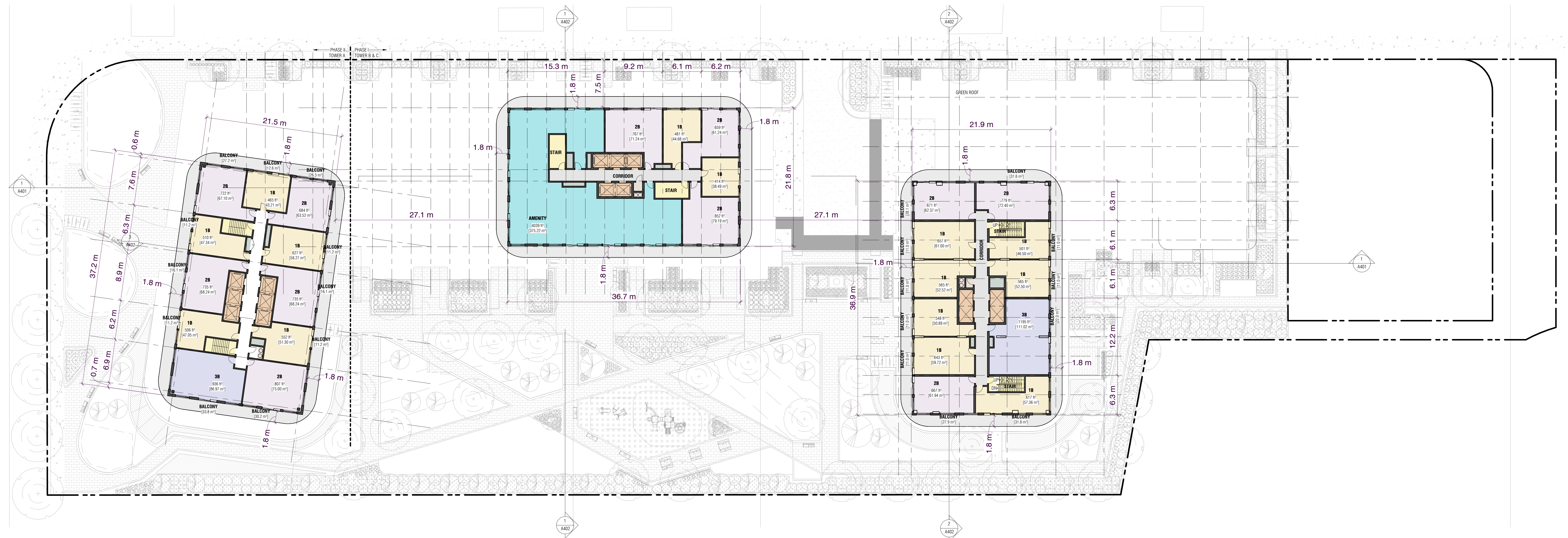
1 Level 8 A104 1:250
