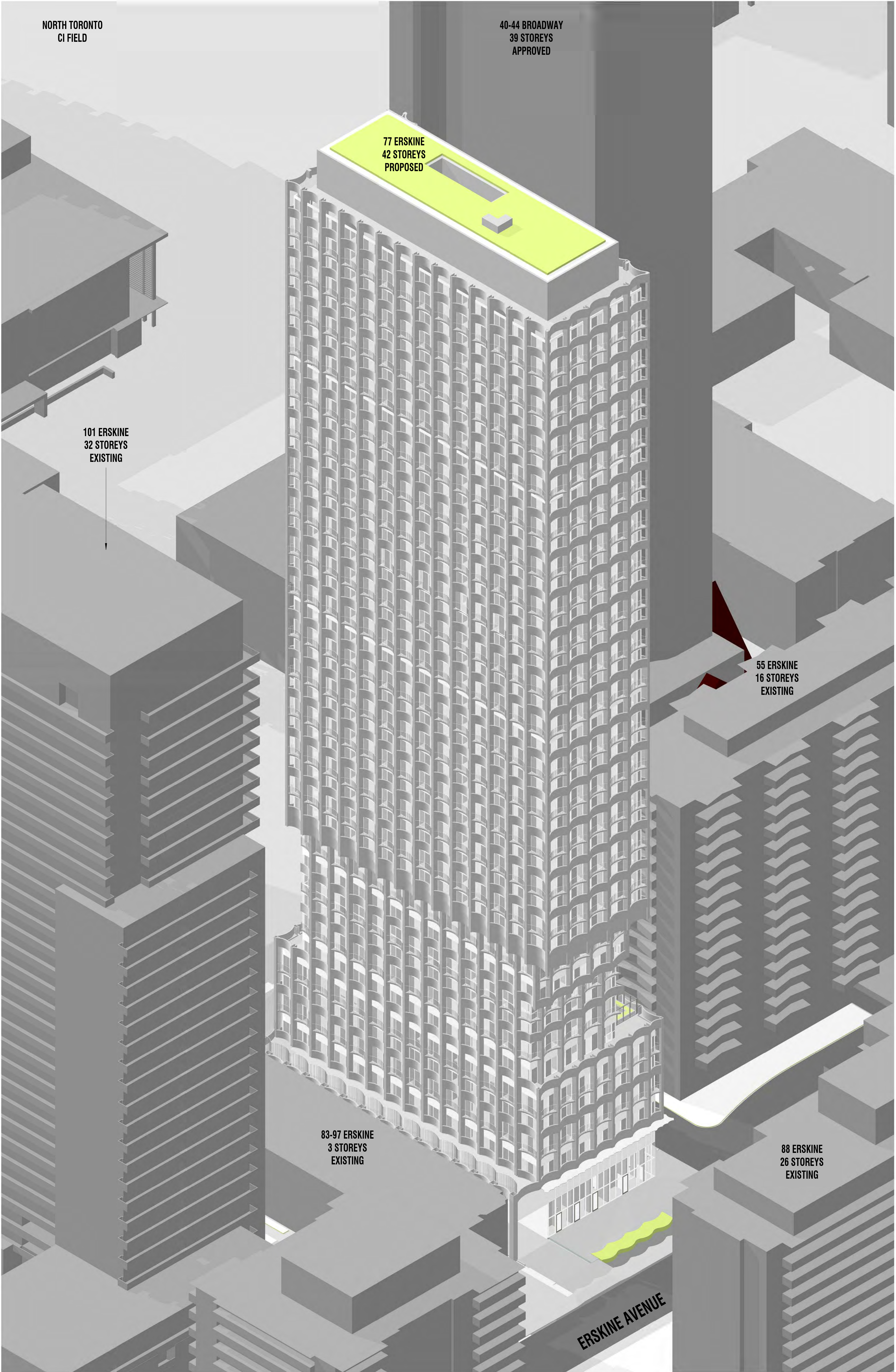
3 MASSING VIEW FROM NORTHEAST A-501
