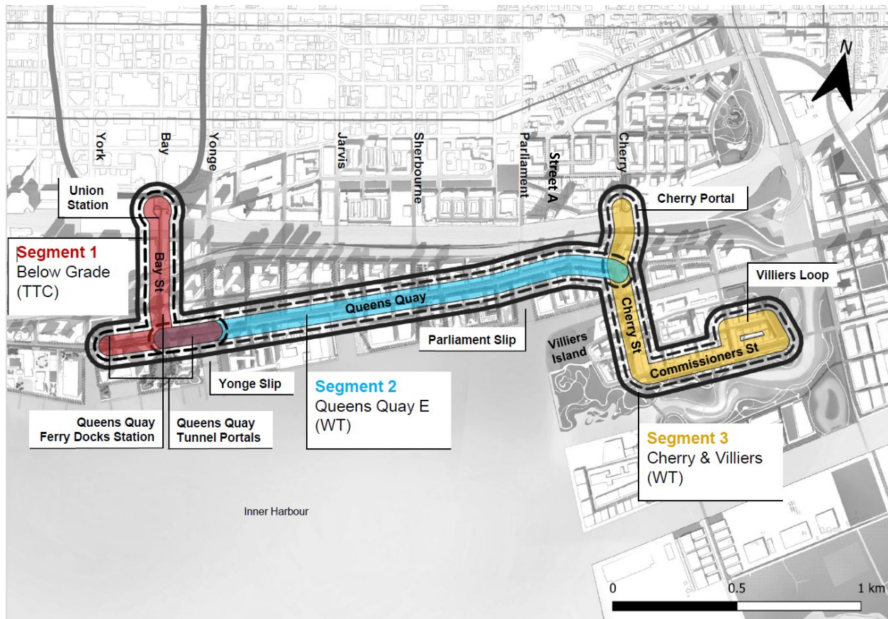
Figure 1. Alignment of the Waterfront East Light Transit Rail Project. Street A shown between Parliament Street and Cherry Street.
