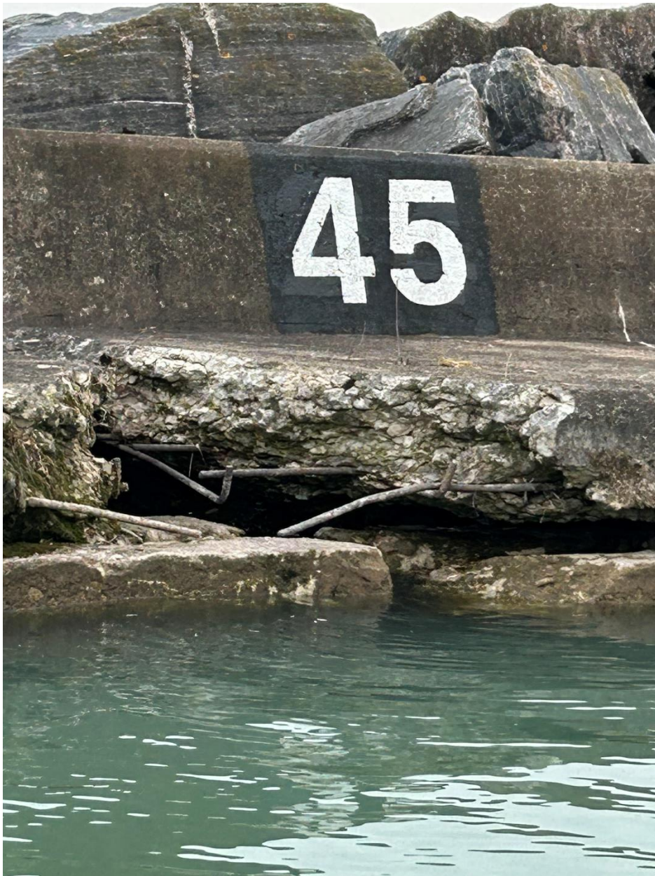
Photo of extensive damage to concrete cap and substructure.
