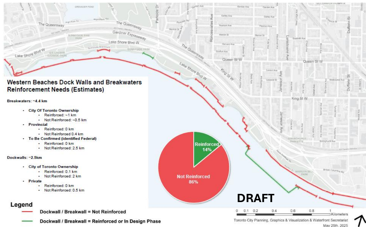
Figure 2: Preliminary mapping of Western Beaches breakwaters reinforcement needs
