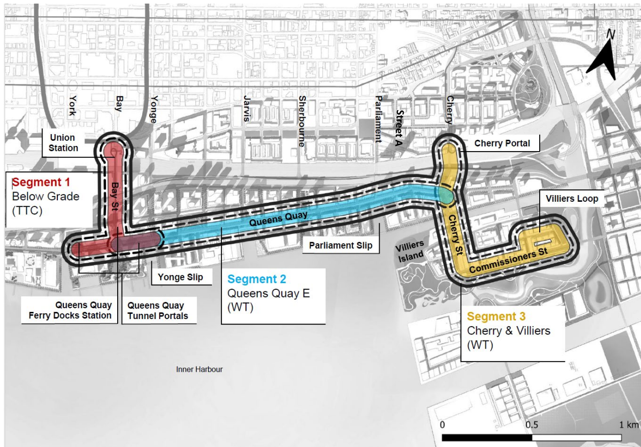
Figure 1. Alignment of the Waterfront East Light Transit Rail Project.
