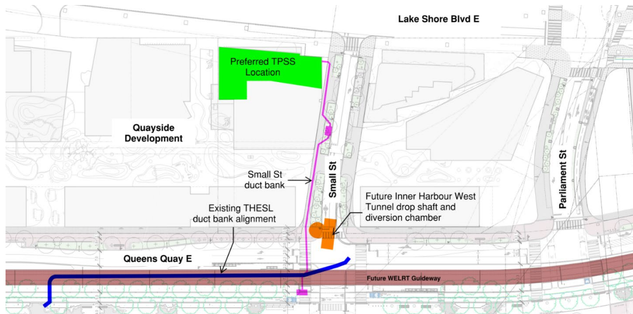
Figure 2. Locations of the duct banks and corresponding infrastructure.
