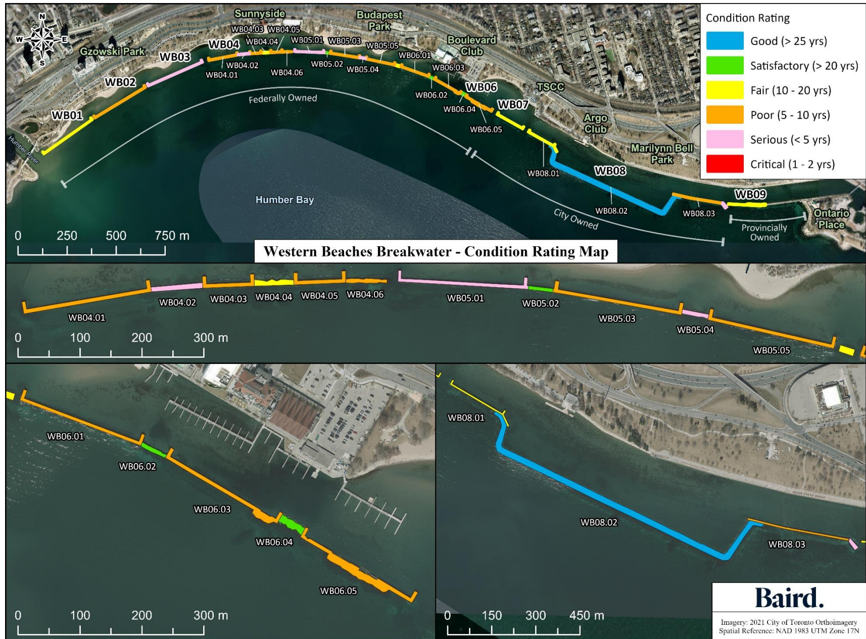
Figure 2: Preliminary mapping of breakwater condition rating ranging from good to critical condition
