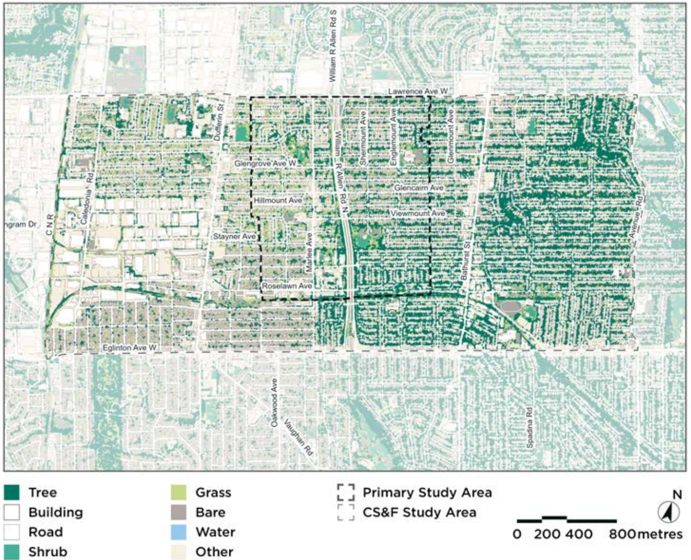
Figure 103 Land cover across the CS&F Study Area.
