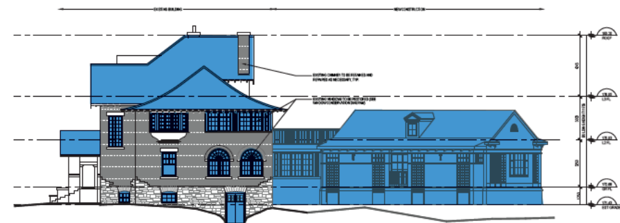
East Elevation
