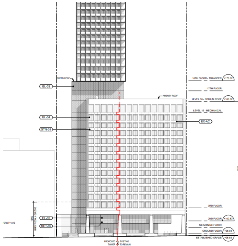
Proposed East Elevation (WZMH Architects)
