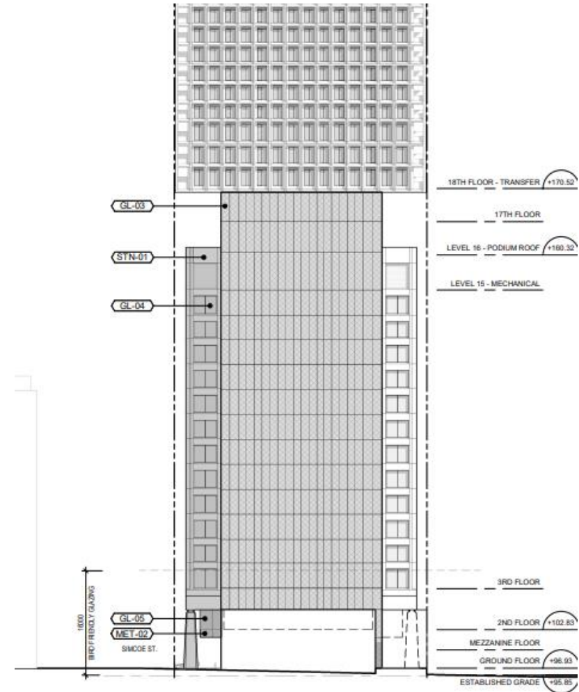
Proposed South Elevation (WZMH Architects)
