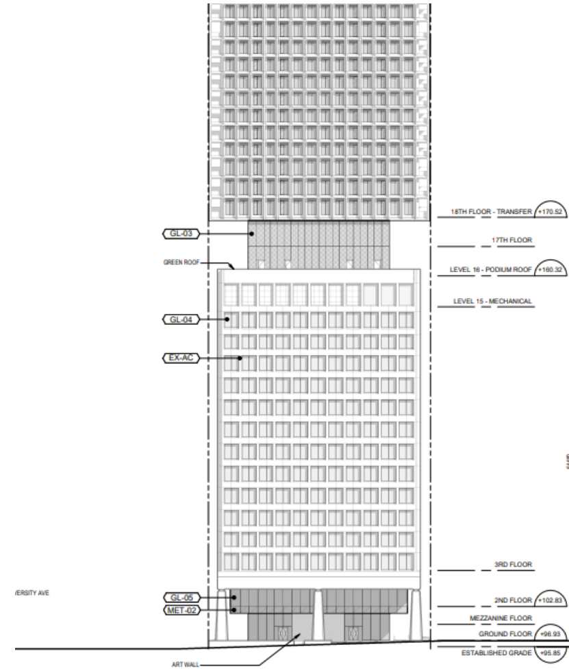
Proposed North Elevation (WZMH Architects)
