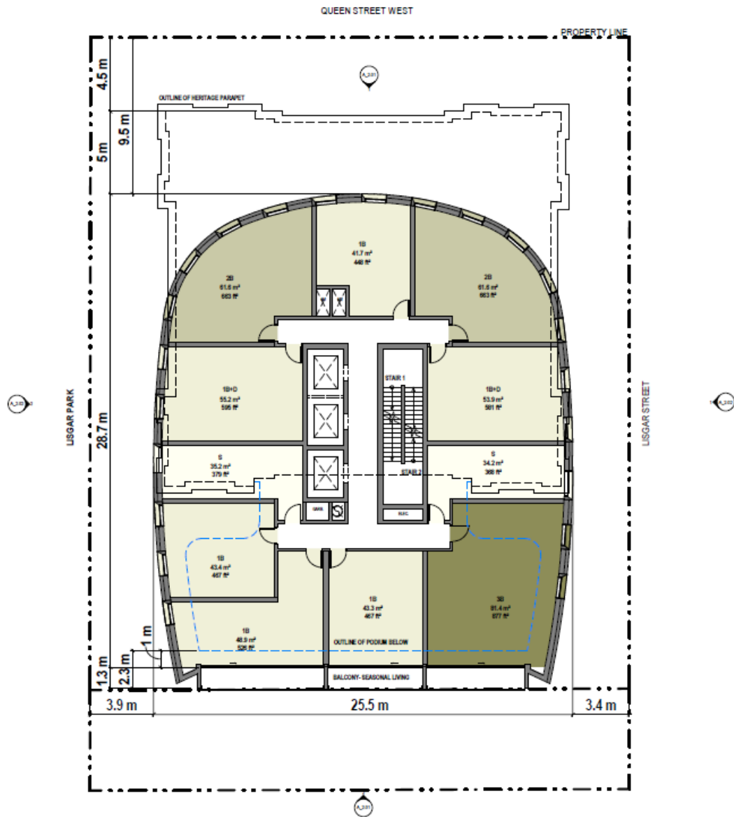
Typical Tower Floor Plan (Level 4-28)
