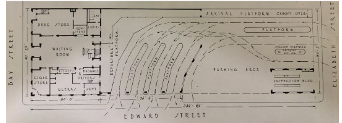
Ground floor plan of terminal building and bus yard ( Construction , April 1932)
