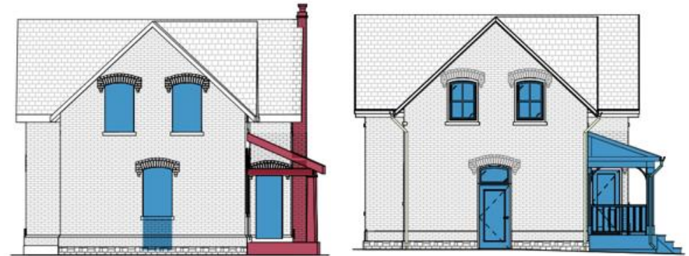
Existing and proposed west elevation of 5933 Steeles Avenue East (ERA Architects Inc.)
