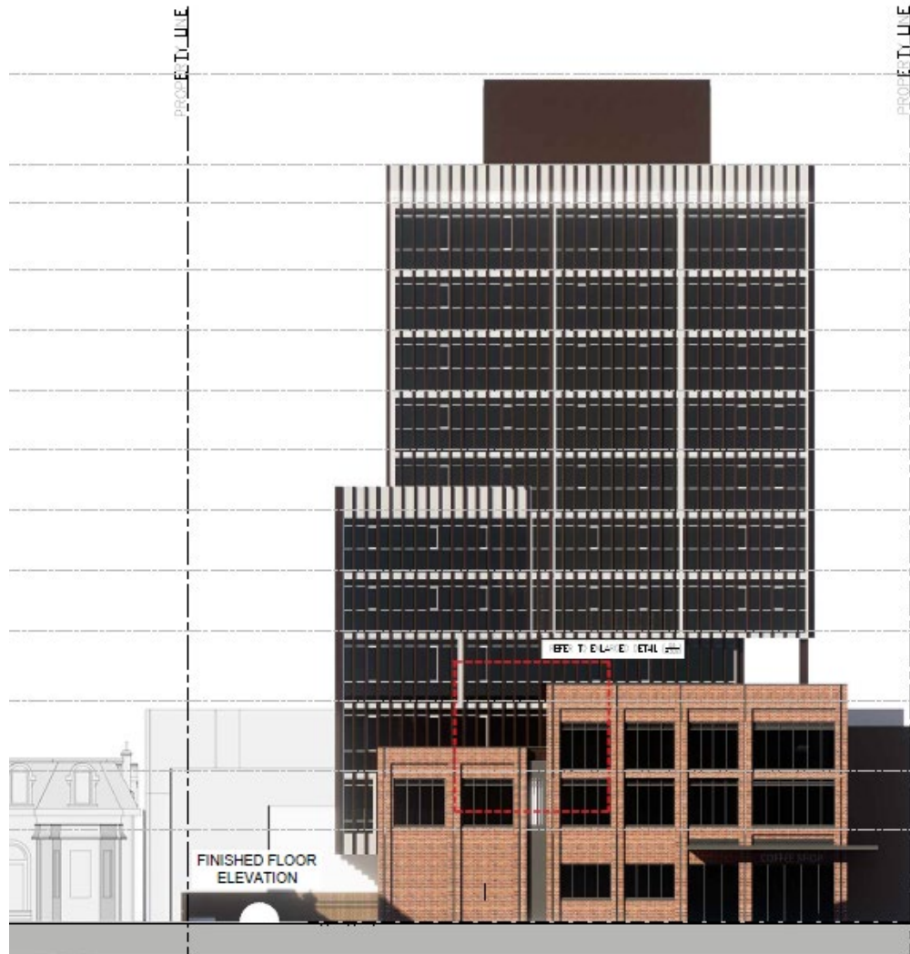
Proposed Bernard Ave Elevation
