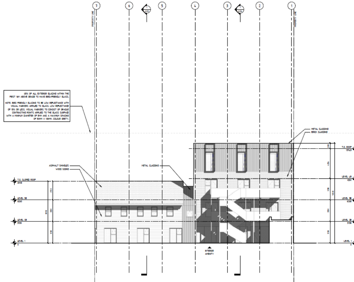
North elevation (Batay-Csorba Architects Inc., June 16, 2025)
