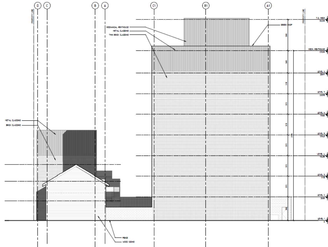
East elevation (Batay-Csorba Architects Inc., June 16, 2025)
