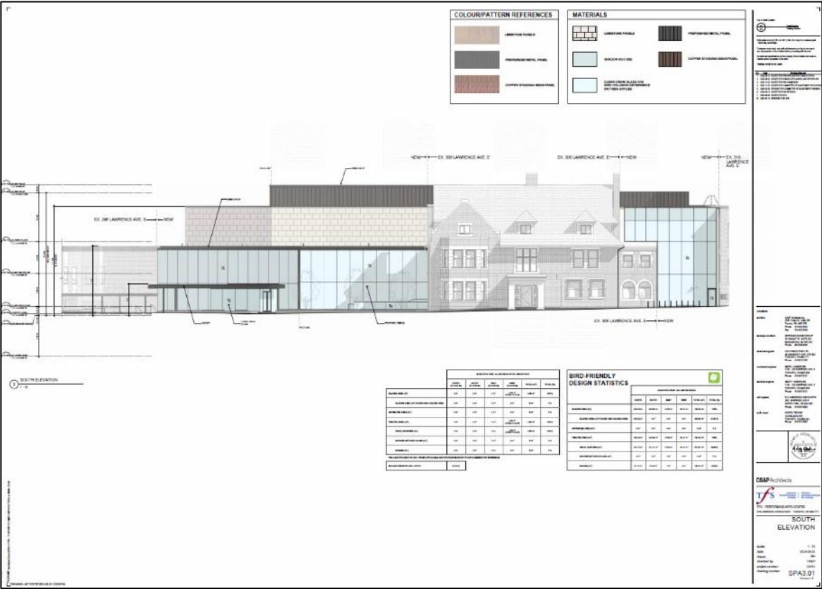
Figure 6: Proposed new auditorium, south elevation (CS+P Architects, Sept 20, 2025).
