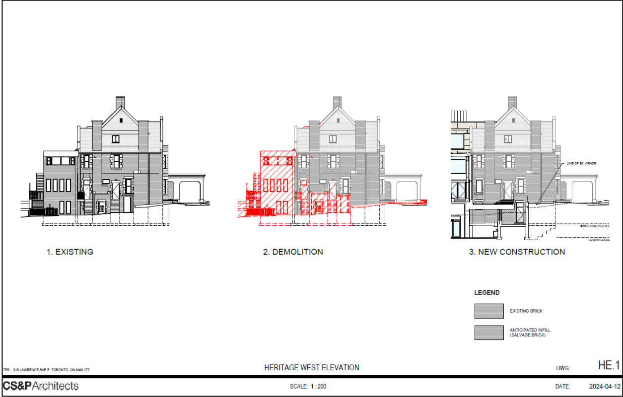
Figure 4 : Demolition Plan of 306 Lawrence Avenue East (CS+P Architect April 12, 2024).
