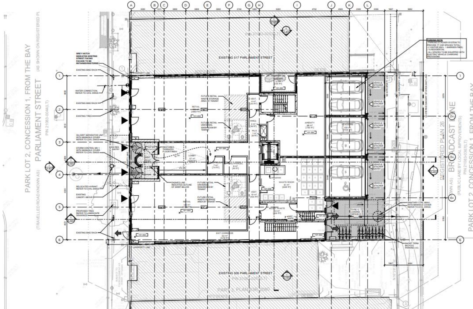
Proposed ground floor of 509 Parliament Street (RAW Architects Inc., 2025).
