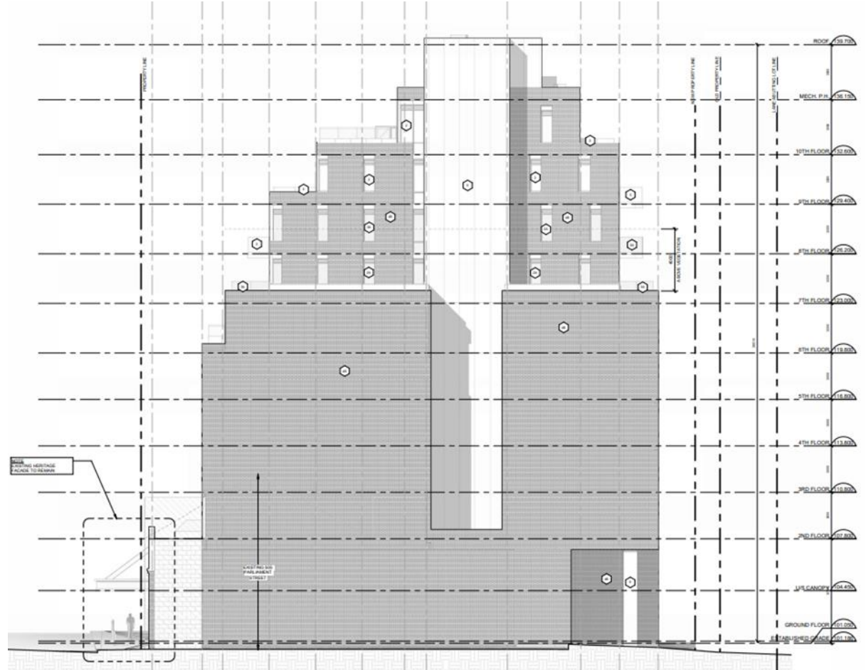
Proposed south elevation of 509 Parliament Street (RAW Architects Inc., 2025).
