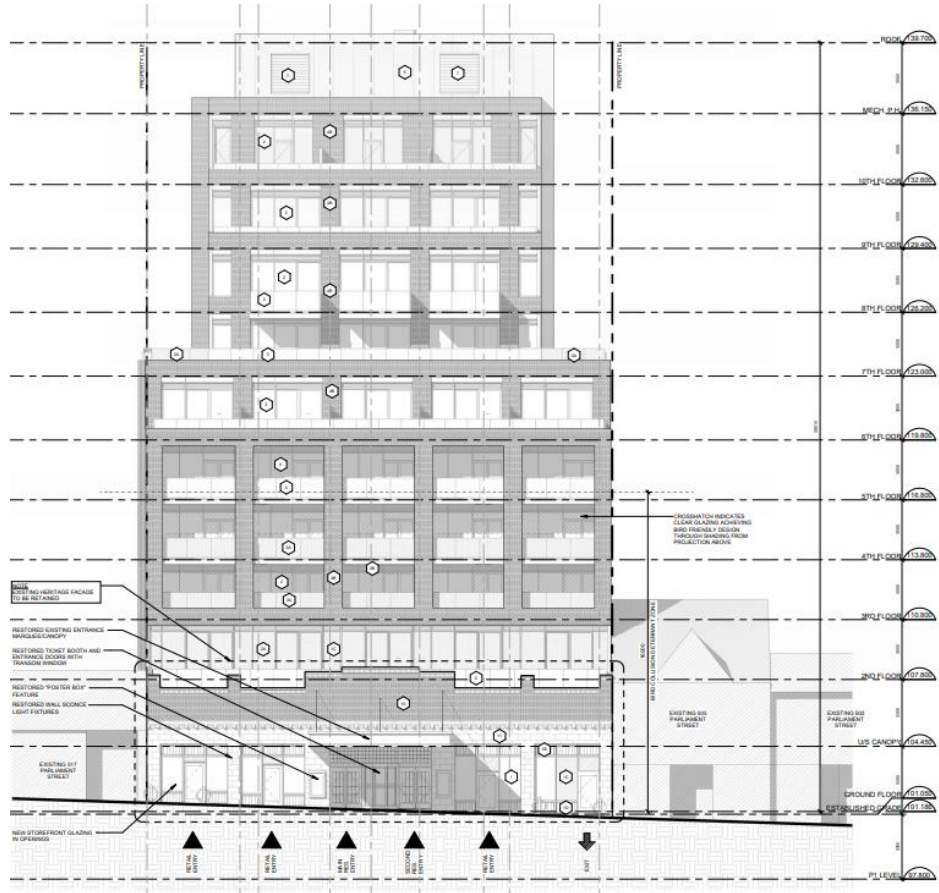
Proposed west elevation of 509 Parliament Street (RAW Architects Inc., 2025).
