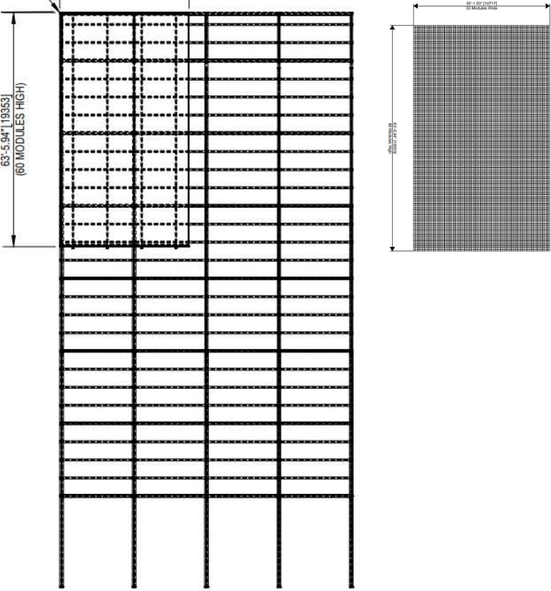
North Elevation
