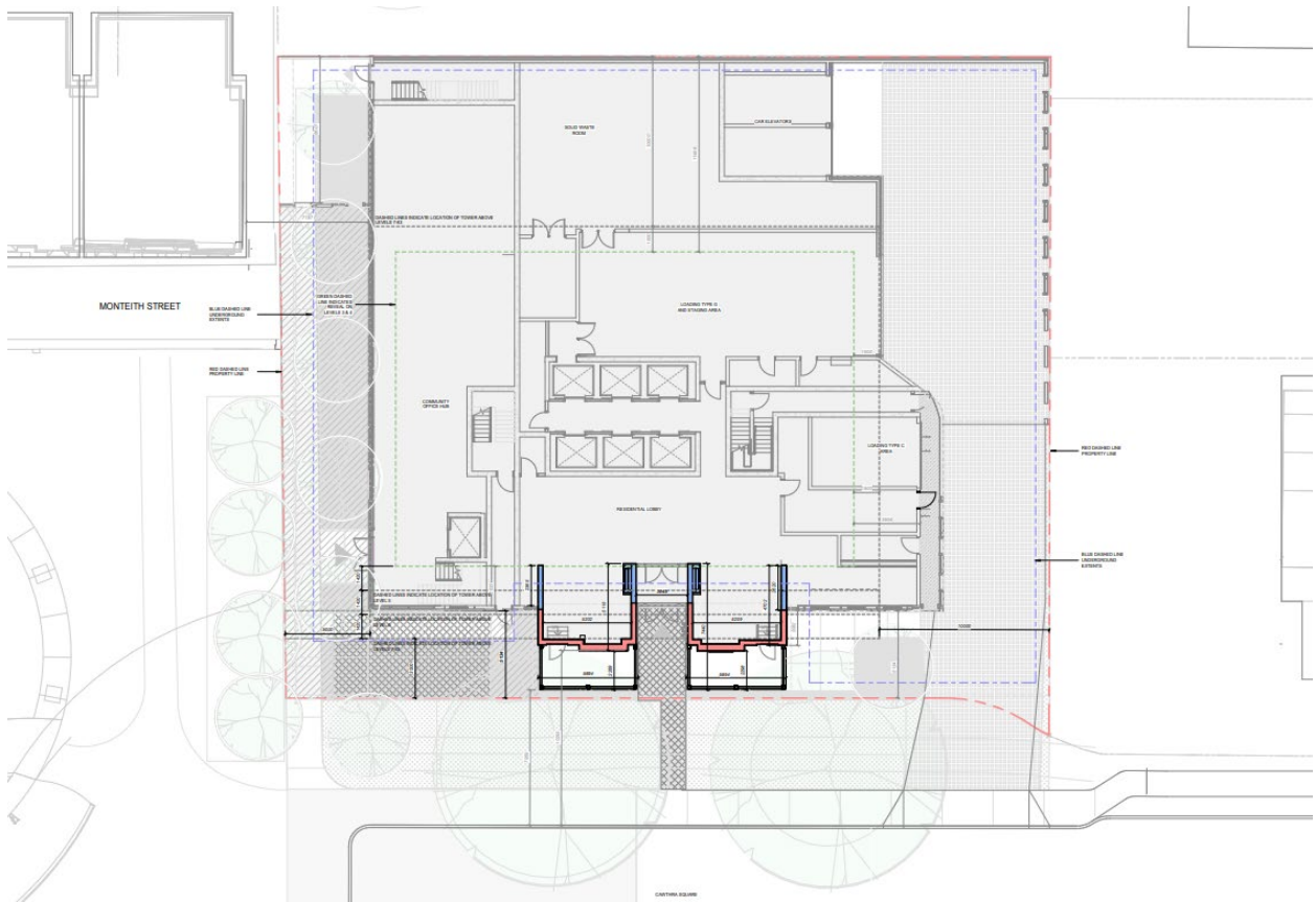
Diagram of 2-12 Cawthra Square showing the portions that are proposed to be retained (red) and reconstructed (blue) (GBCA Architects Ltd., 2024).
