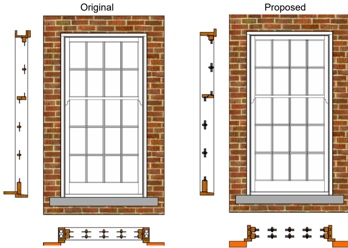
Architectural drawing showing original (left) window elevation and proposed (right) (Browne & Perry Joinery Co.).
