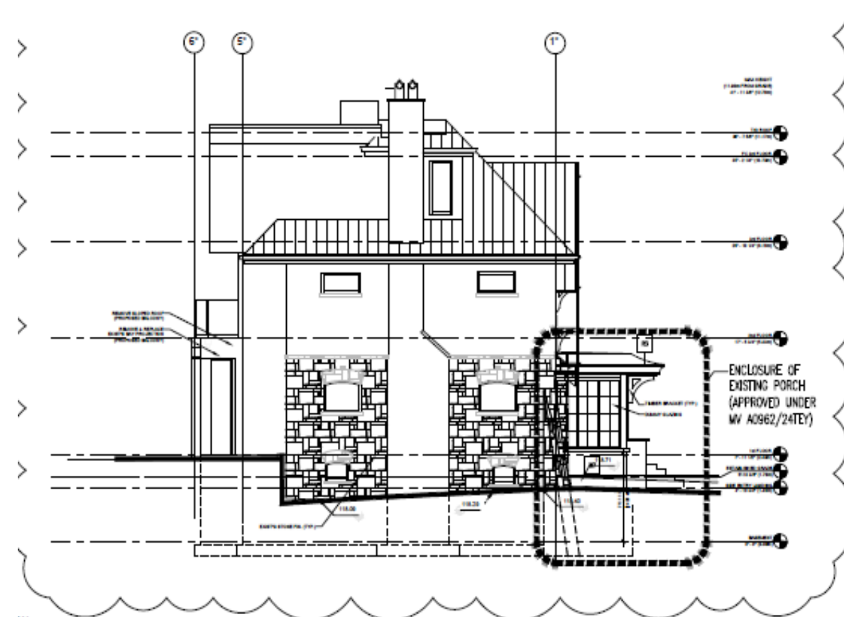
Proposed side, east elevation of 21 Baby Point Crescent (Starkey Group Architects Inc., 2025).
