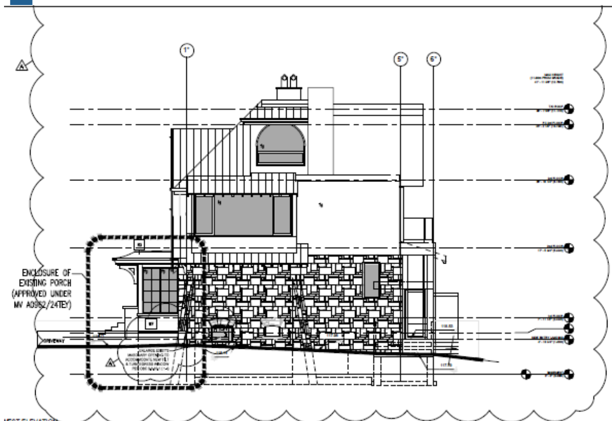
Proposed side, west elevation of 21 Baby Point Crescent (Starkey Group Architects Inc., 2025).
