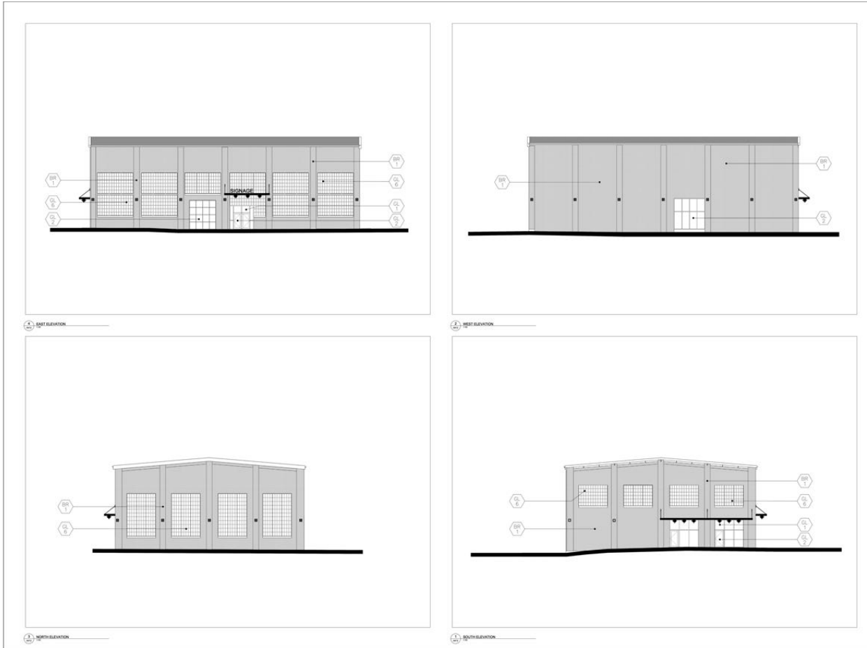
Figure 20: Proposed west, east, north, and south elevations of 153 Eastern Avenue (Cleaning Room building) (Core Architects Inc., 2026).
