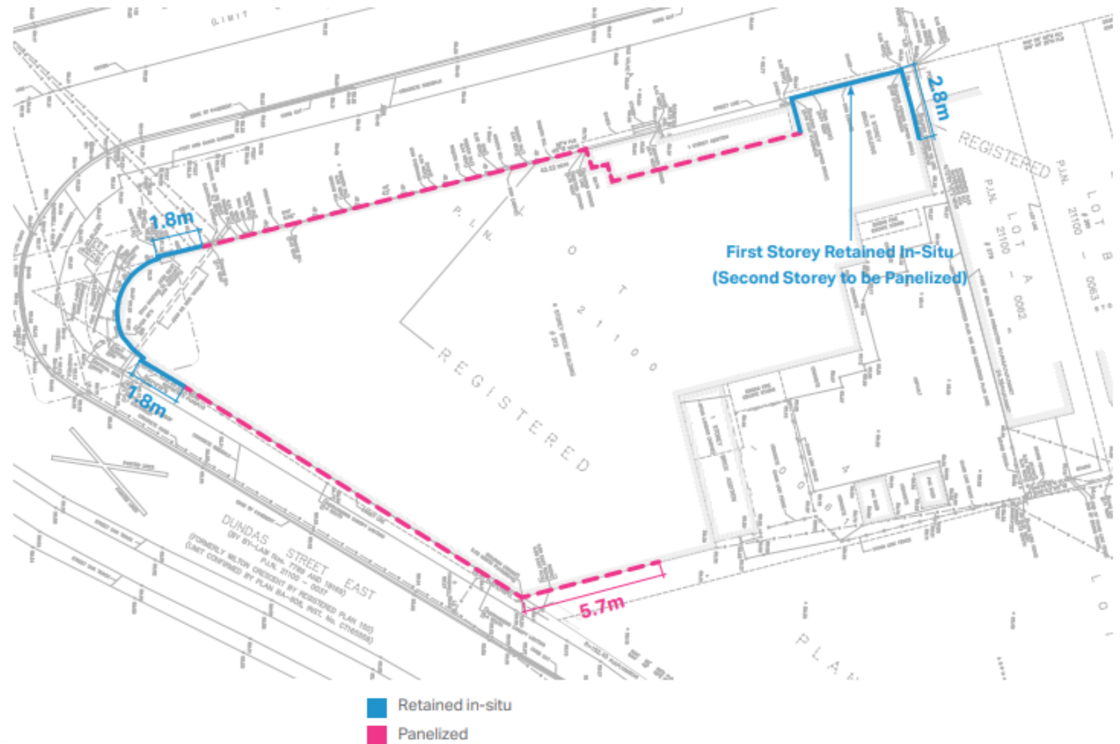
Diagram showing retained and panelized elevations (Giaino + Associates Architects Inc., April 16, 2026).
