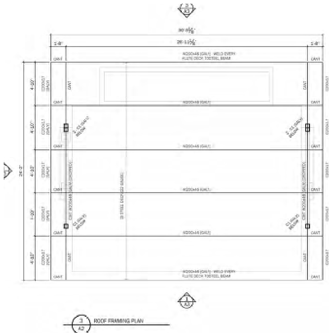
Proposed roof framing plan of detached carport at 79 Whitehall Road (Christopher Walker Architect, 2026).
