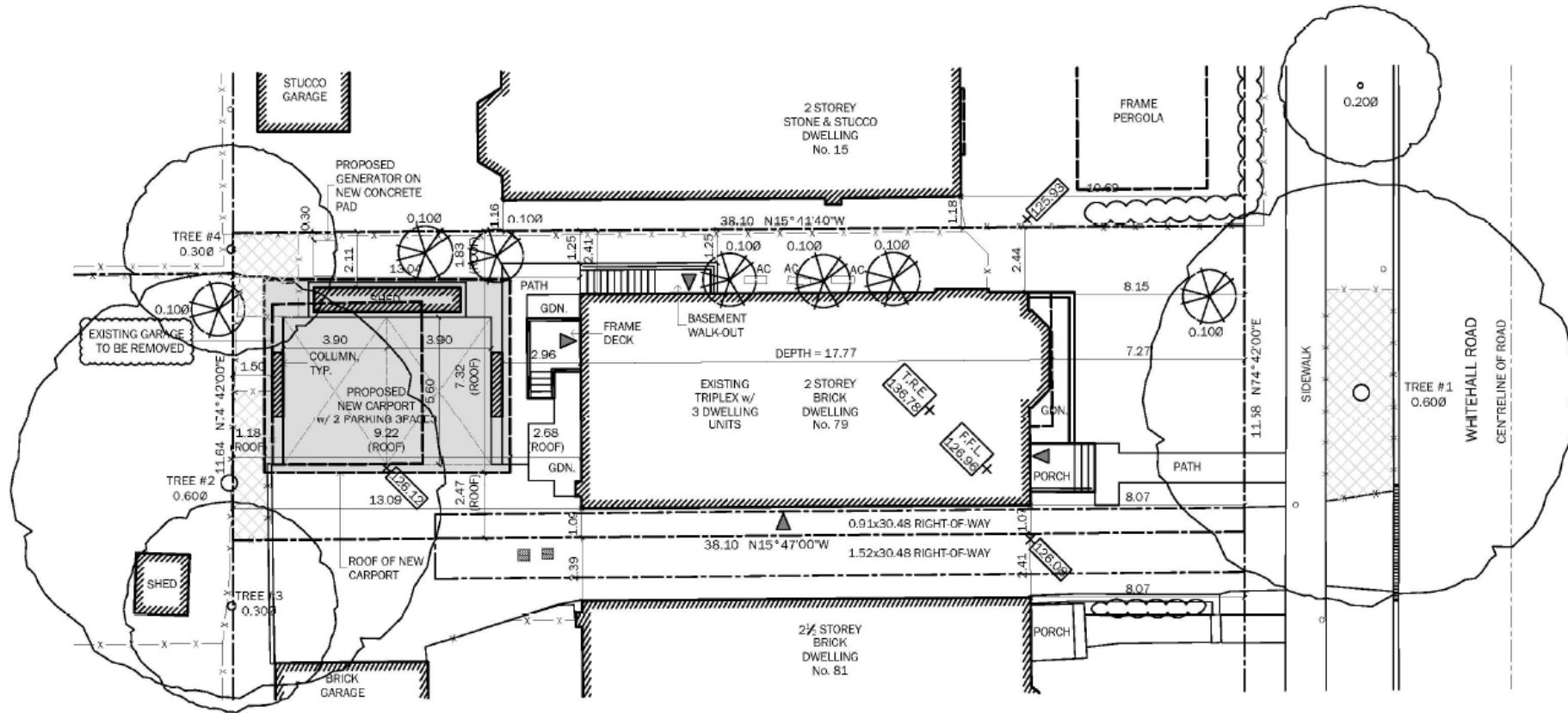
Proposed site plan of 79 Whitehall Road (Christopher Walker Architects, 2026)
