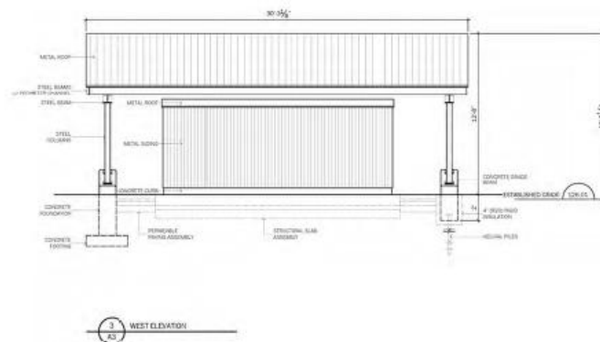
Proposed elevations of new structure at 79 Whitehall Road (Christopher Walker Architects, 2026)
