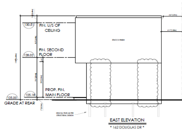
Proposed elevations of new structure at 162 Douglas Drive (House Lab Inc, 2026)
