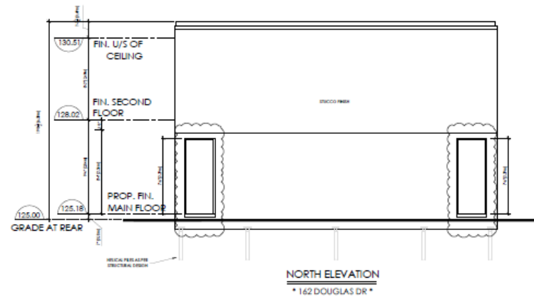
Proposed elevations of new structure at 162 Douglas Drive (House Lab Inc, 2026)
