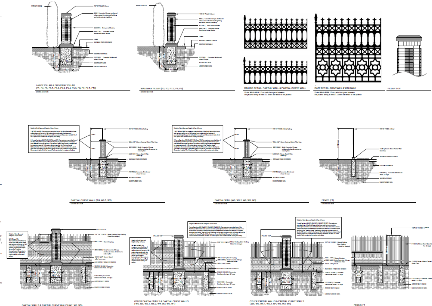
Proposed landscape details, elevations and cross sections (bsq Landscape Architects, 2026)
