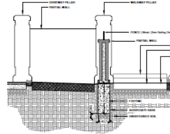
GLEN ROAD ENTRANCE WALKWAY PARTIAL WALL
