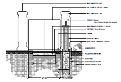
GLEN ROAD ENTRANCE WALKWAY
