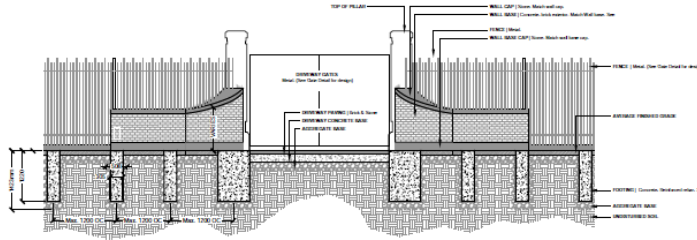
WHITNEY AVENUE DRIVEWAY ENTRANCE WALL
