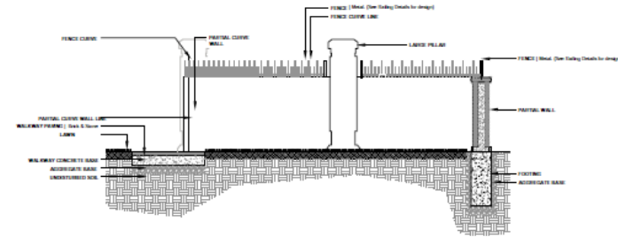
GLEN ROAD WALKWAY PARTIAL CURVE WALL (W1)
