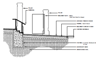
WHITNEY AVENUE ENTRANCE STEPS
