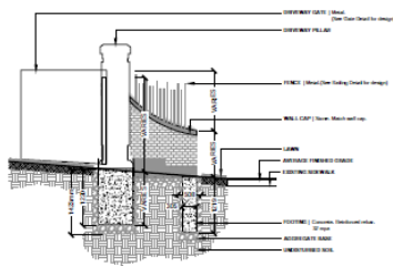
WHITNEY AVENUE DRIVEWAY ENTRANCE WALL
