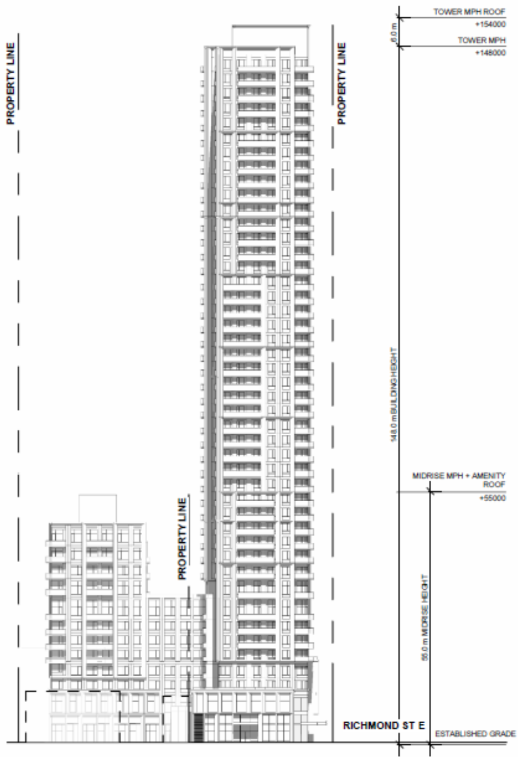
West Elevation
