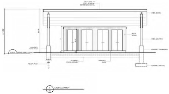
Proposed elevations of detached carport at 79 Whitehall Road (Christopher Walker Architect, 2026).
