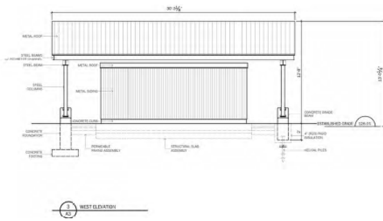
Proposed elevations of detached carport at 79 Whitehall Road (Christopher Walker Architect, 2026).
