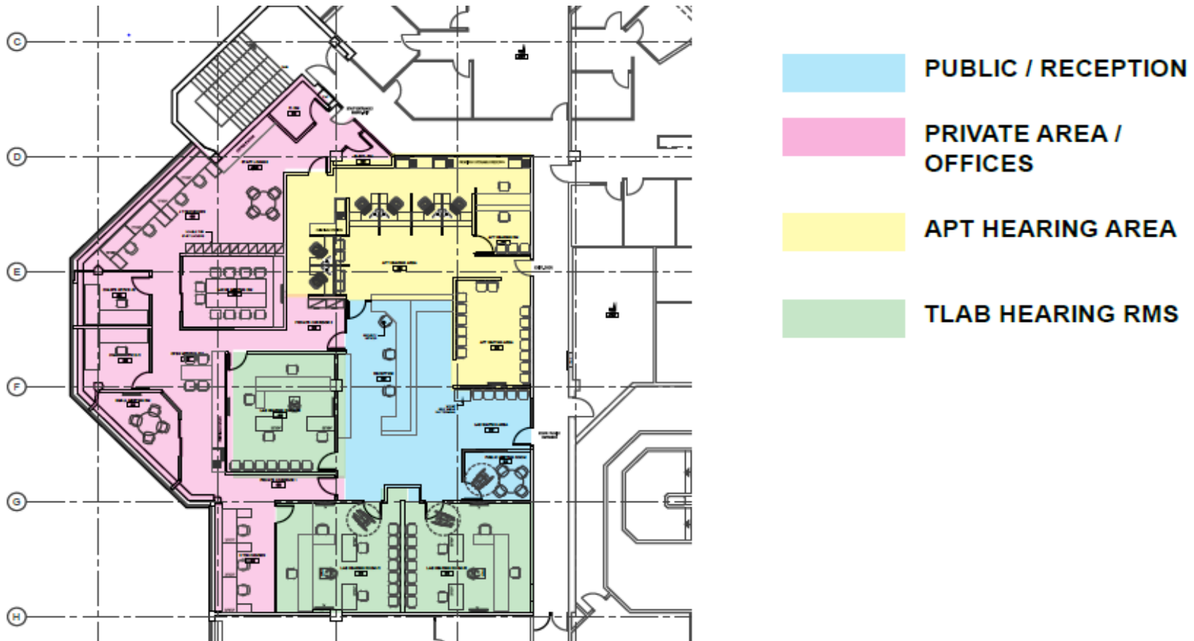
FURNITURE PLAN
