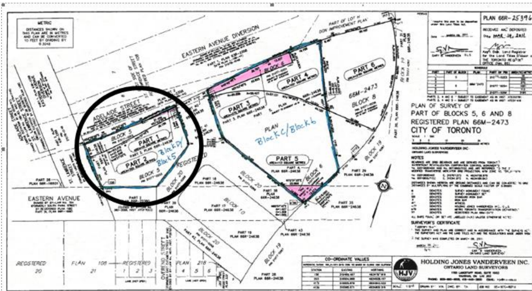
Plan 66R-25396
