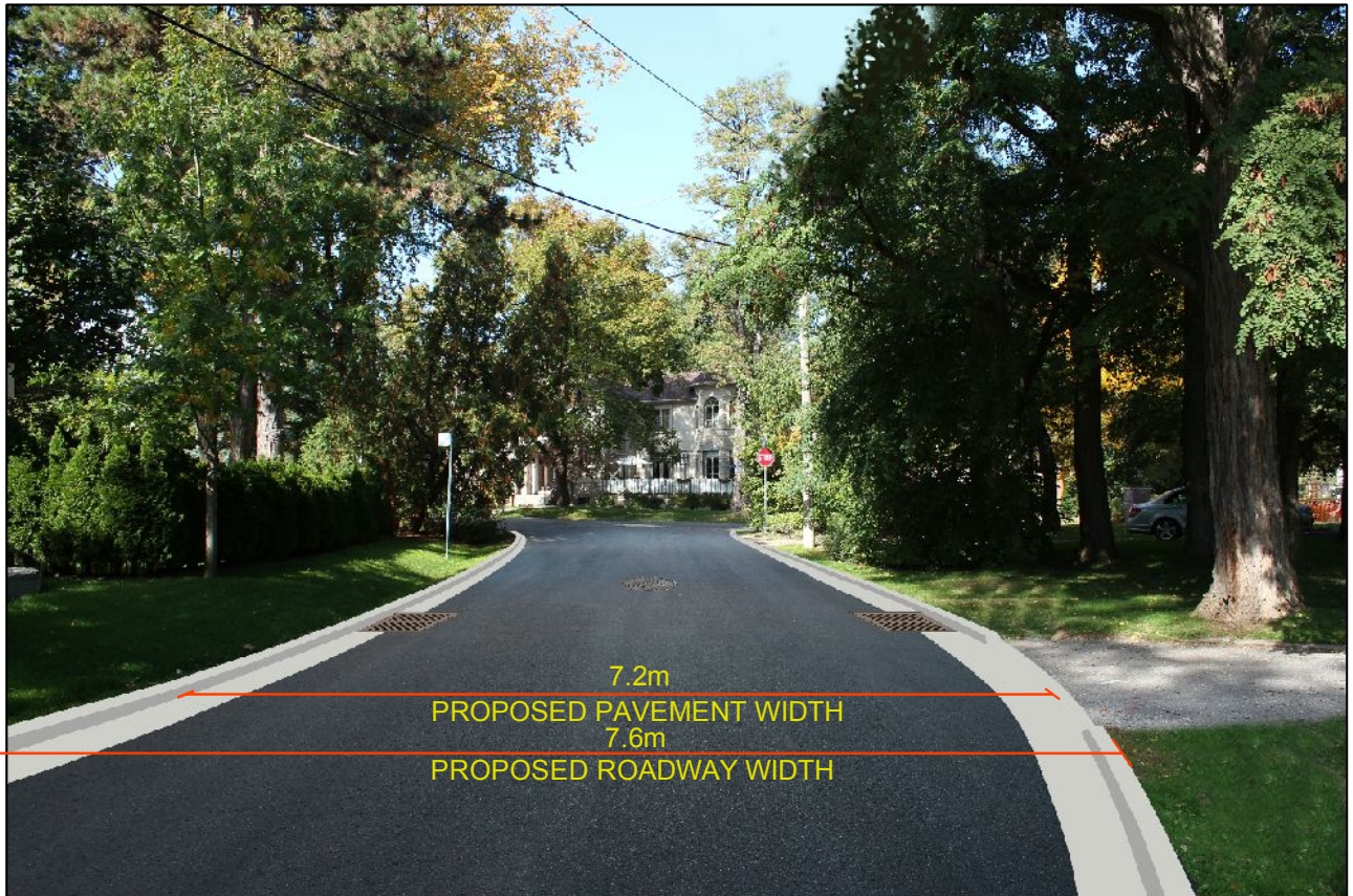
FIGURE LE2 ILLUSTRATION OF EXISTING AND PROPOSED ROAD DIMENSIONS - LEWES CRES
