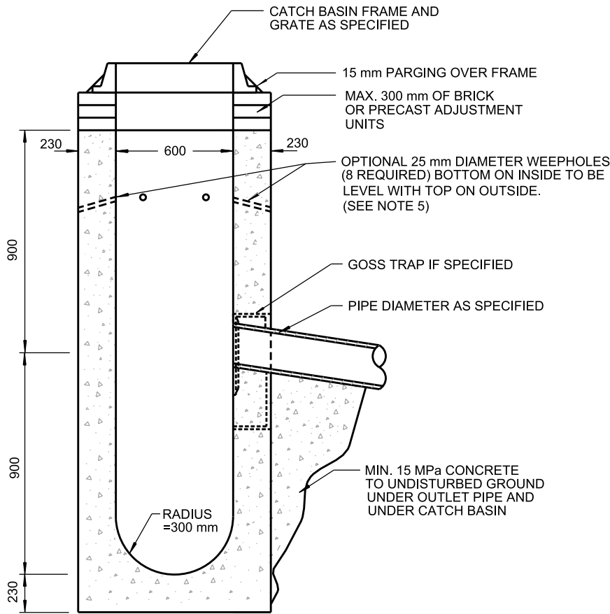
SECTION A
