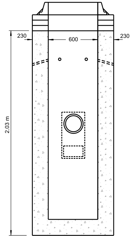
SECTION B
