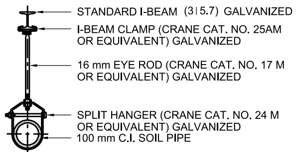
SECTION N
