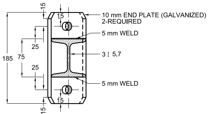
SECTION O
