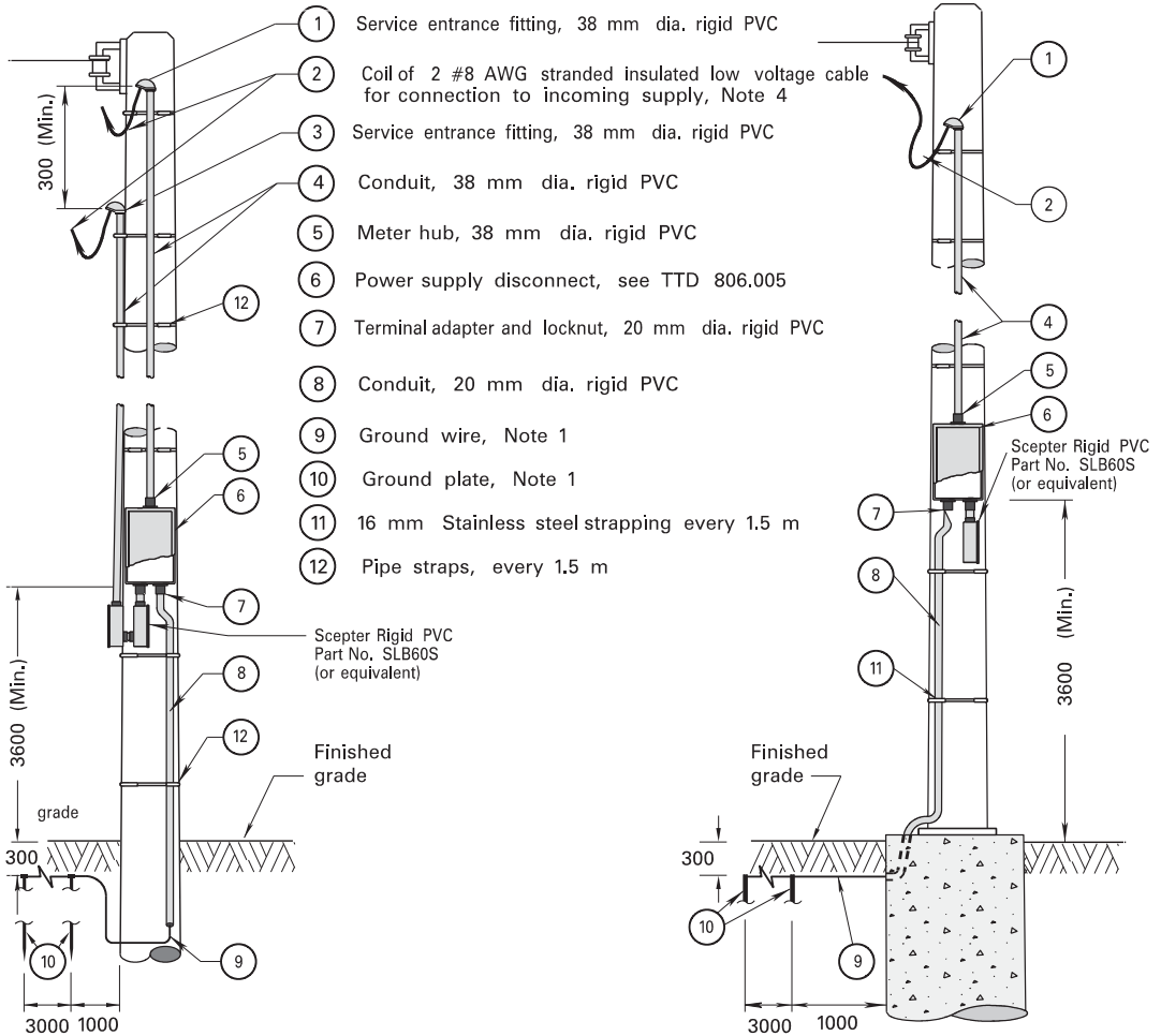
OVERHEAD SUPPLY INSTALLATION ON A DIRECT BURIED POLE
