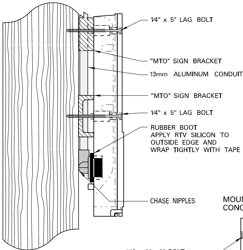
MOUNTING ON A WOOD POLE
