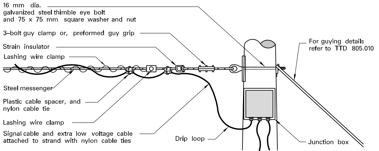
DEAD END ATTACHMENT
