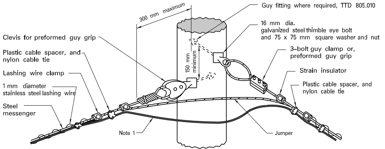
ANGLE POLE ATTACHMENT Line Angle Greater Than 30 degrees
