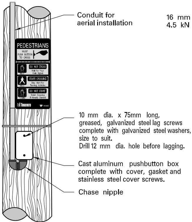
MOUNTING ON WOOD POLE OR TRAFFIC POLE
