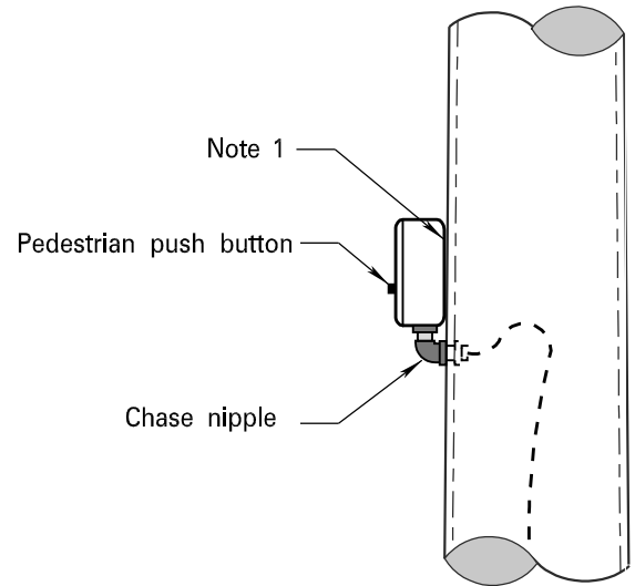
MOUNTING ON STEEL POLE
