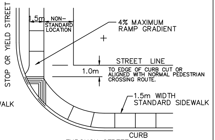
THROUGH STREET CURB CUT AND SIDEWALK RAMP AT LOCAL STREETS
