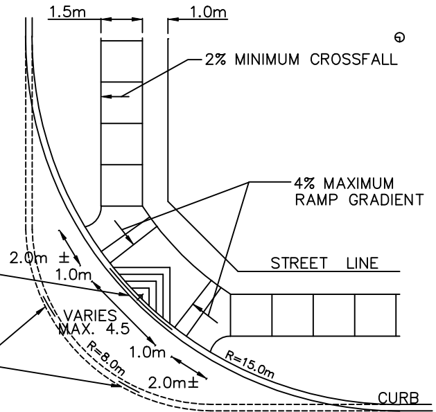
CURB CUT AND SIDEWALK RAMP AT MAJOR FOUR-WAY STOP OR SIGNAL CONTROLLED INTERSECTIONS
