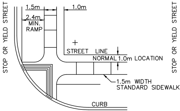
THROUGH STREET CURB CUT AND SIDEWALK RAMP AT LOCAL STREETS
