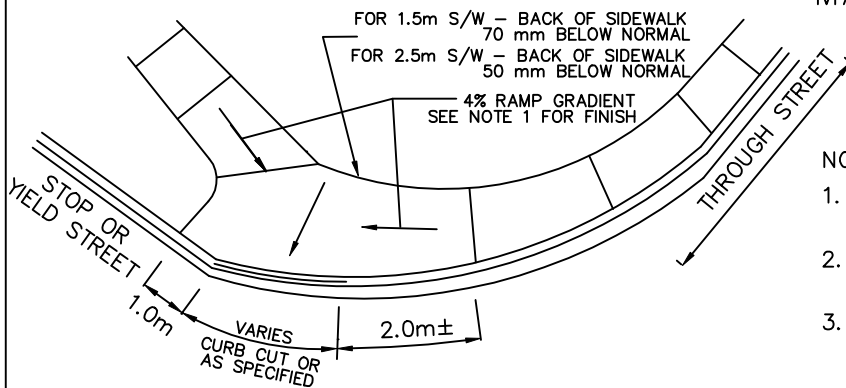
TYPICAL VIEW OF SIDEWALK RAMP
