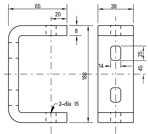
BRACKET 'C'
