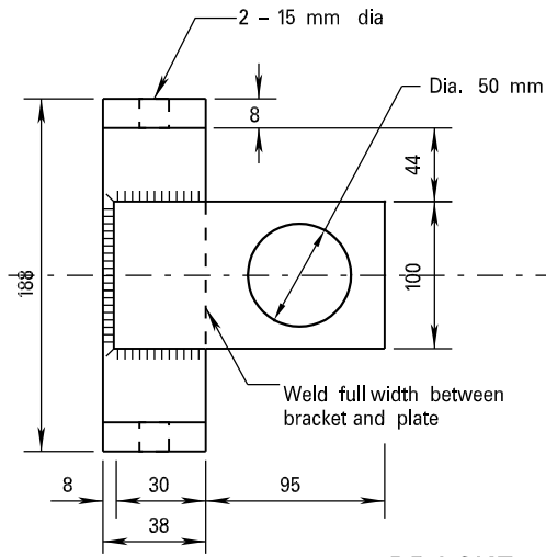
BRACKET 'A'
