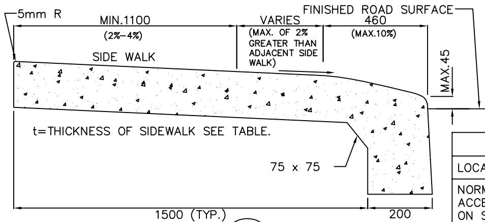
SECTION A
