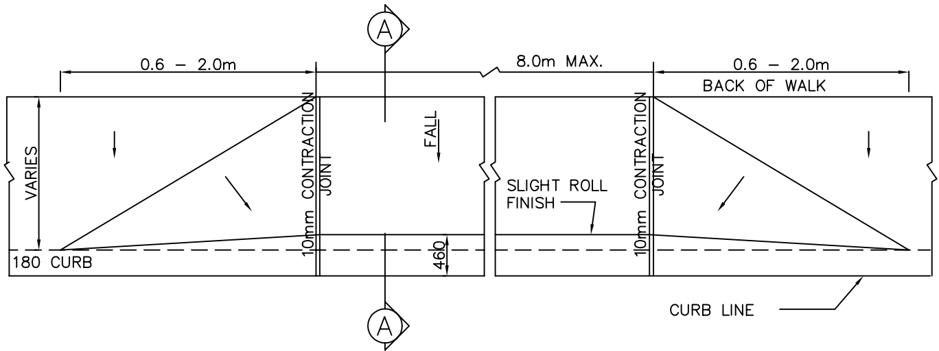
PLAN
