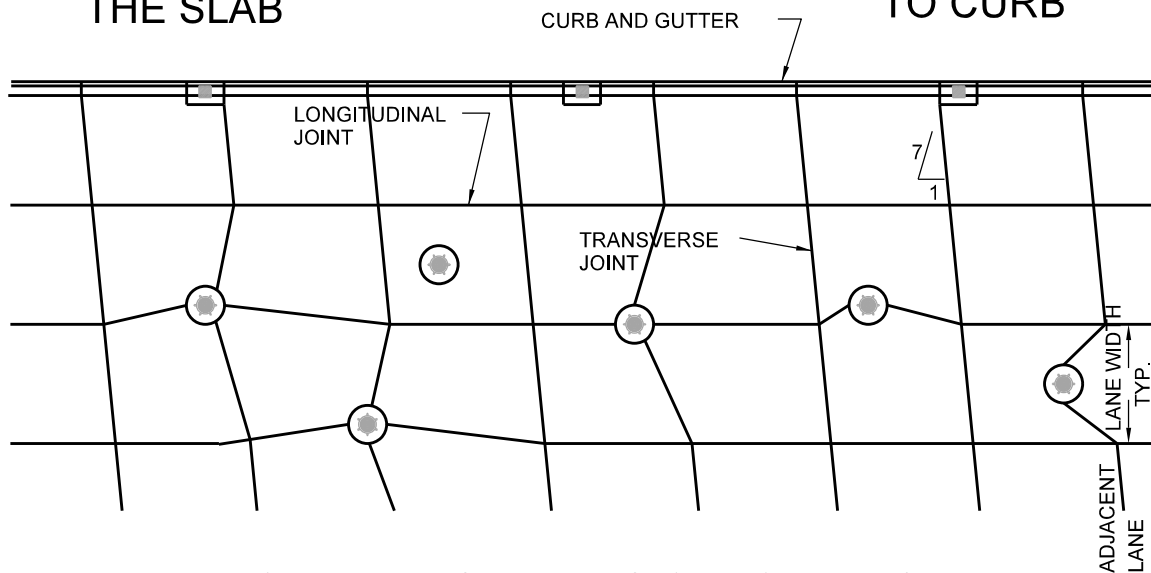
TYPICAL ADJUSTMENTS OF JOINTING AT UTILITY ISOLATION
