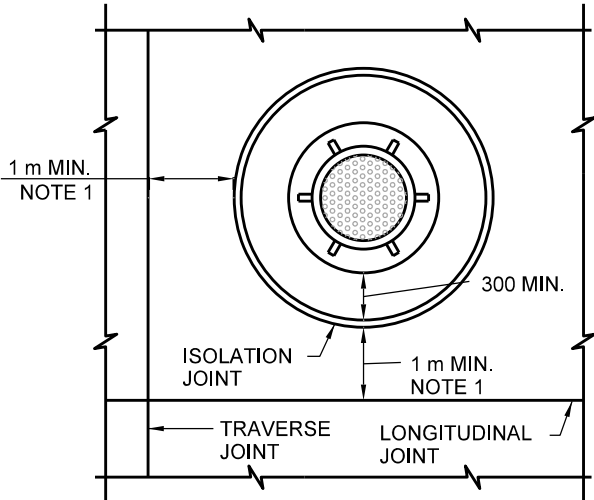
ISOLATION WITHIN THE SLAB
