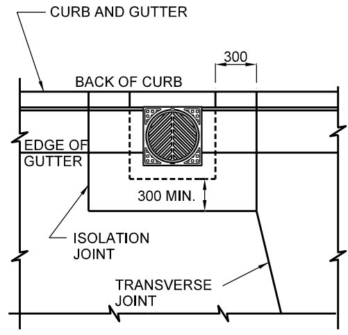
ISOLATION ADJACENT TO CURB
