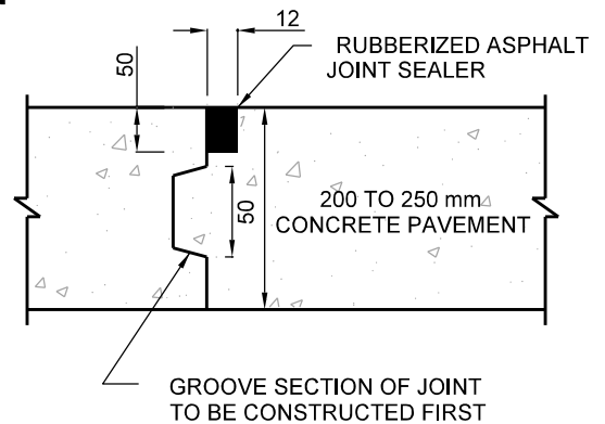
ISOLATION JOINT
