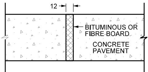
EXPANSION JOINT
