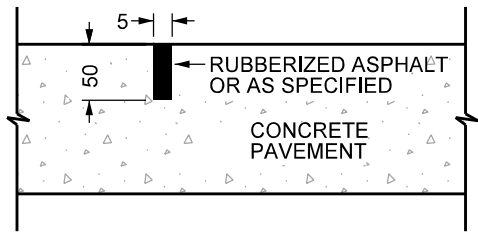
CONTRACTION JOINT
