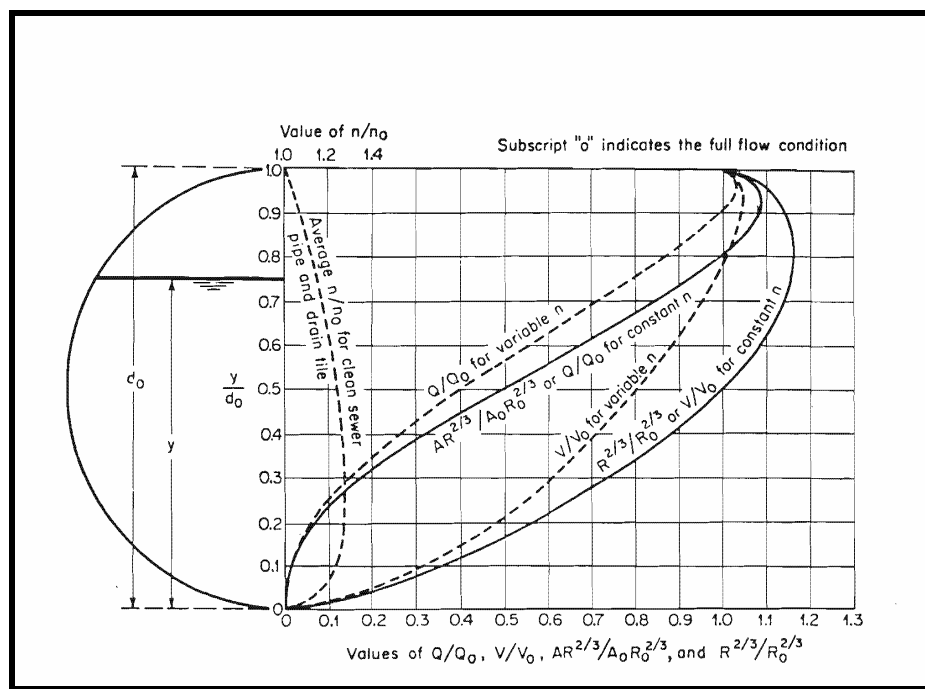
Figure: Hydraulic elements graph for circular pipe
