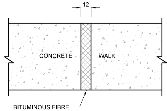
TYPICAL EXPANSION JOINT
