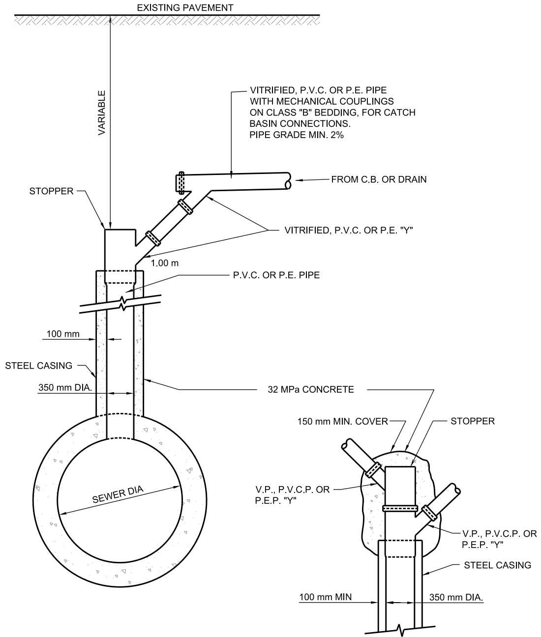
ALTERNATIVE CONNECTION
