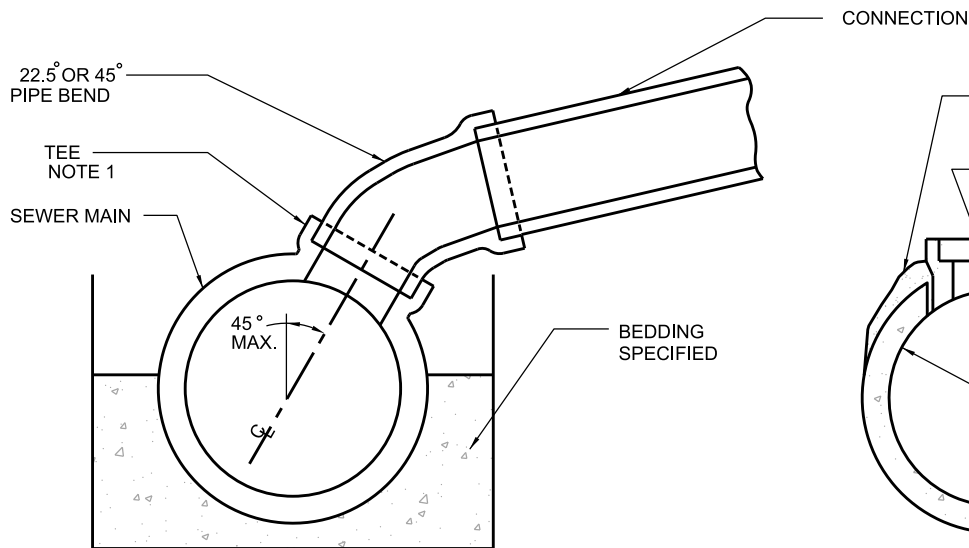
CONNECTION WITHOUT RISER
