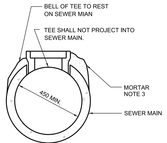
FIELD INSTALLED TEE FOR CONCRETE CONNECTIONS
