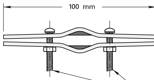
6 mm x 25 mm medium thread Nut and Bolt JB CLAMP DETAIL
